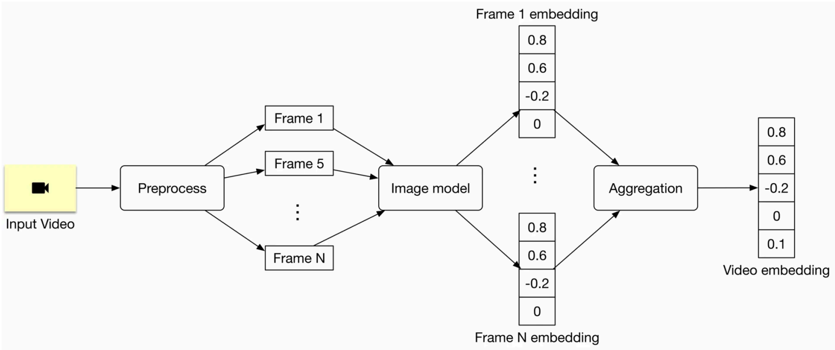
Figure 4.17: A frame-level model
