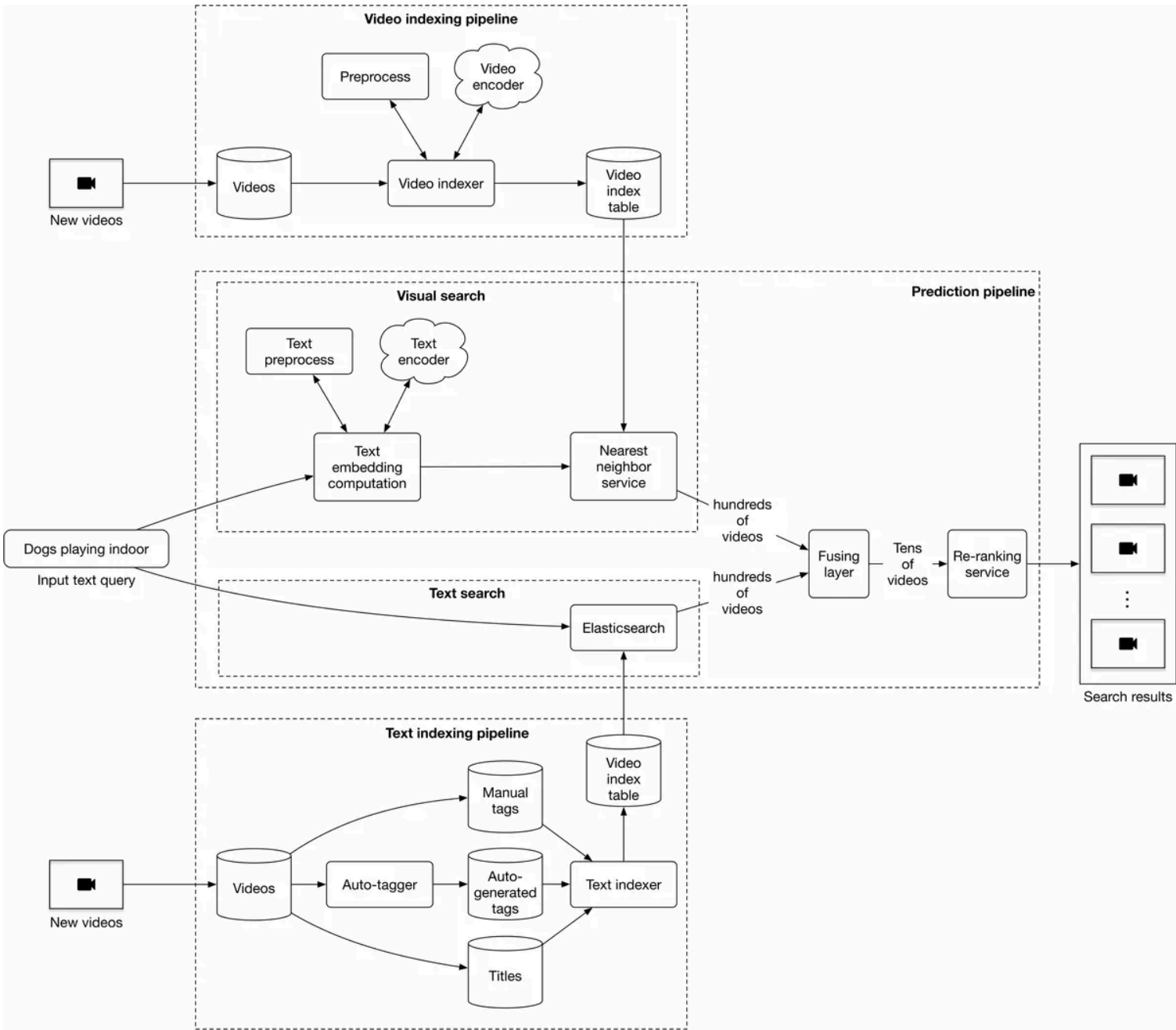
Figure 4.19: ML system design
