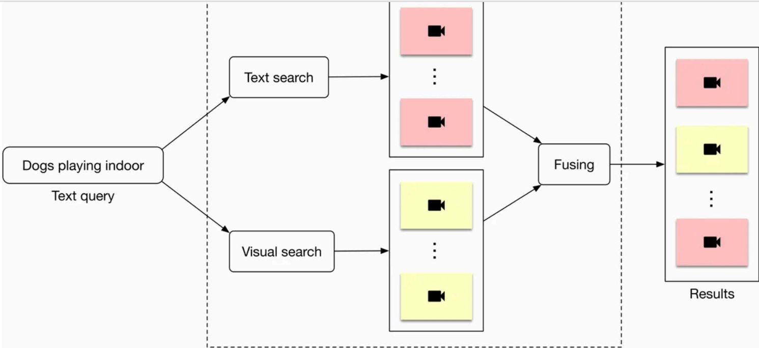
Figure 4.3: High-level overview of the search system
