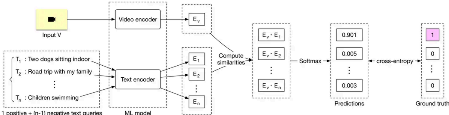
Figure 4.18: Loss computation
