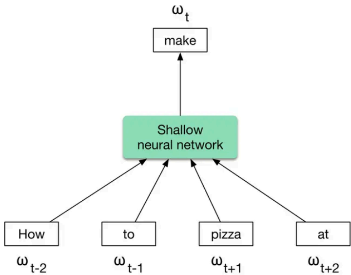
Figure 4.14: CBOW approach
