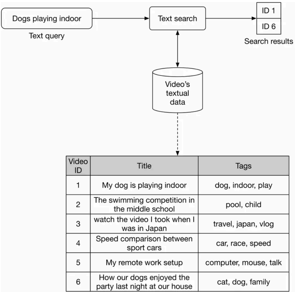
Figure 4.5: Text search
